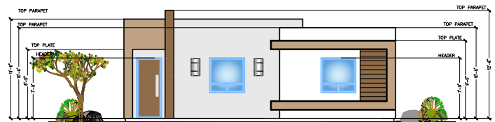
Front Elevation
