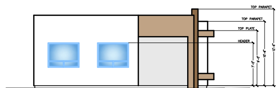
Left Elevation
